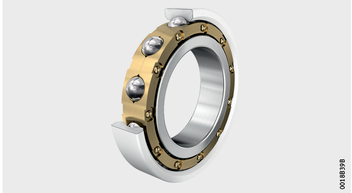
Figure 4 Current-insulated deep groove ball bearing 6215-M-j20AA
