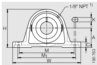
AK Housing
