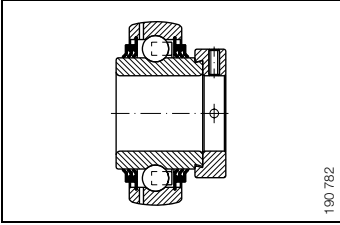
Figure 1 · Triple Lip Seal
