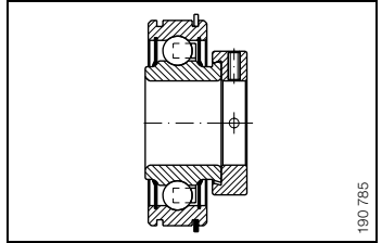
Figure 4 · Cylindrical O.D.
