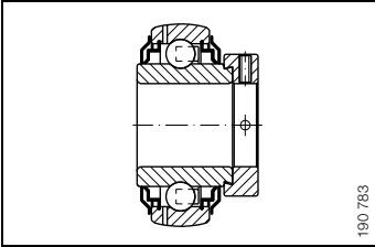
Figure 2 · Anti-Wrap Flinger Shield
