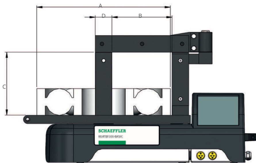
63 Rozmery HEATER50 do HEATER200
