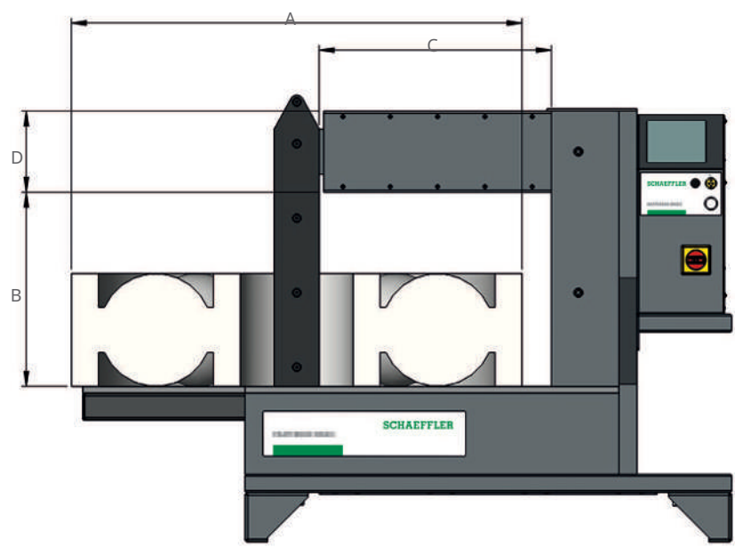
65 Rozmery HEATER800 a HEATER1600
