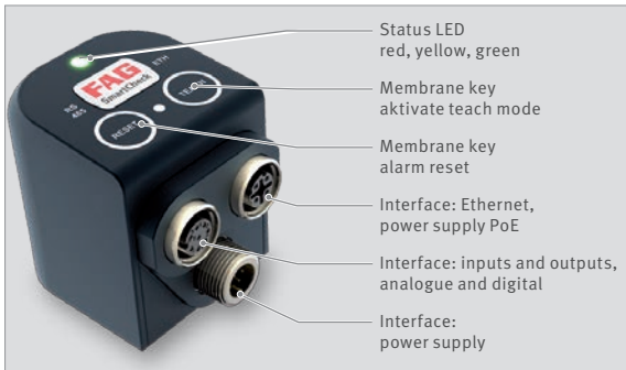
Operating elements and interfaces of FAG SmartCheck
