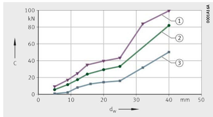
Figure 4 Dynamic load carrying capacity – PWG, RGT, KGT
