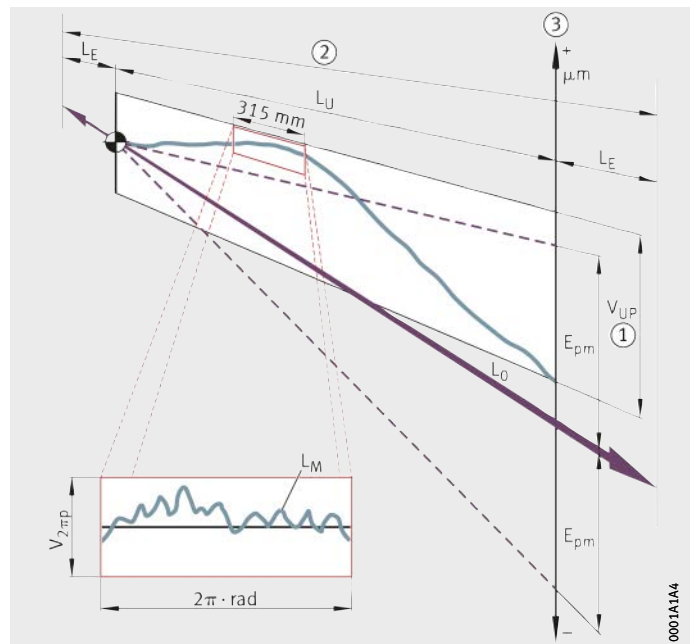
Figure 2 Diagram of pitch deviation
