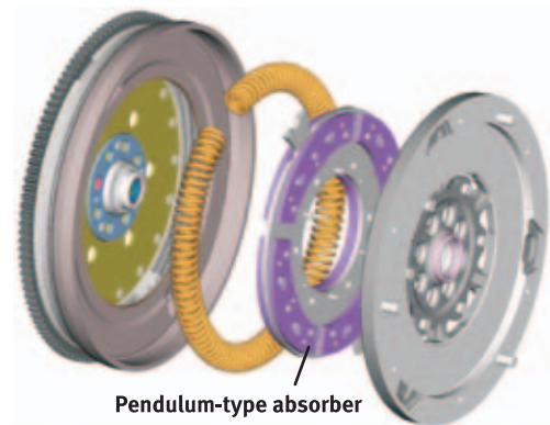
Figure 28 Design realization of a DMF with secondary-side centrifugal pendulum-type absorber
