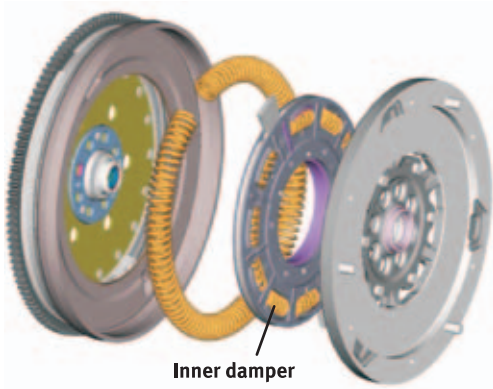
Figure 19 Components of a DMF with inner damper
