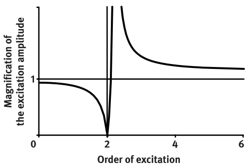
Figure 27 Theoretical transfer function of a centrifugal pendulum-type absorber
