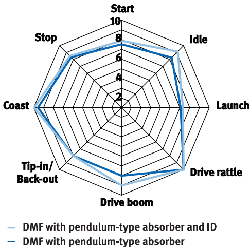
Figure 32 Comparison between centrifugal pendulum-type absorbers, inner and outer with additional ID
