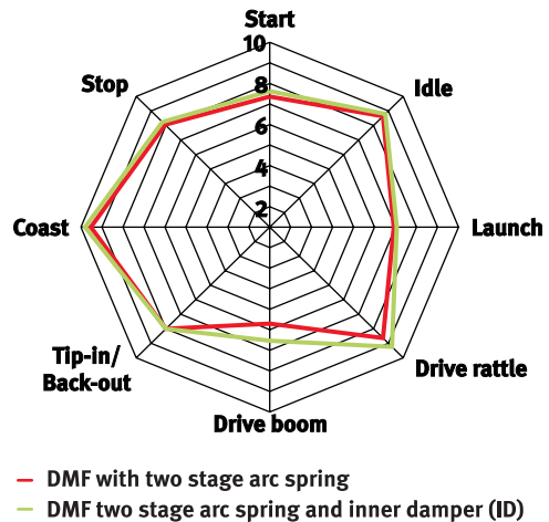
Figure 22 Comparison of DMF with and without inner damper
