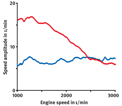
Figure 30 Comparison of test results between a conventional DMF with inner damper and a DMF with centrifugal pendulum-type absorber
