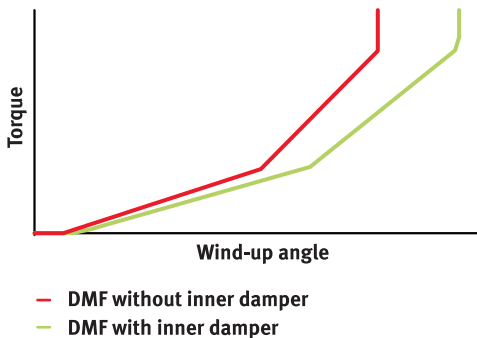
Figure 20 Comparison of spring characteristics of DMF with and without inner damper
