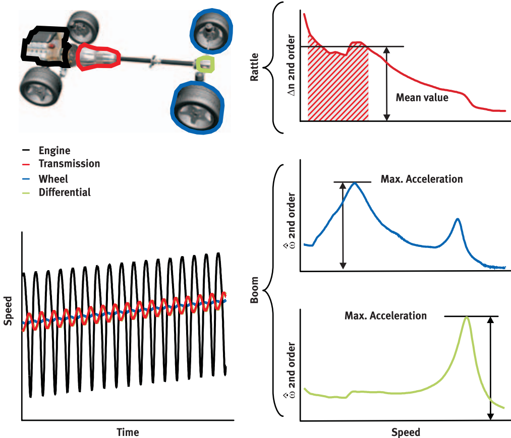
Figure 6 Full load in drive mode: Analysis of the metrics for rattle and boom
