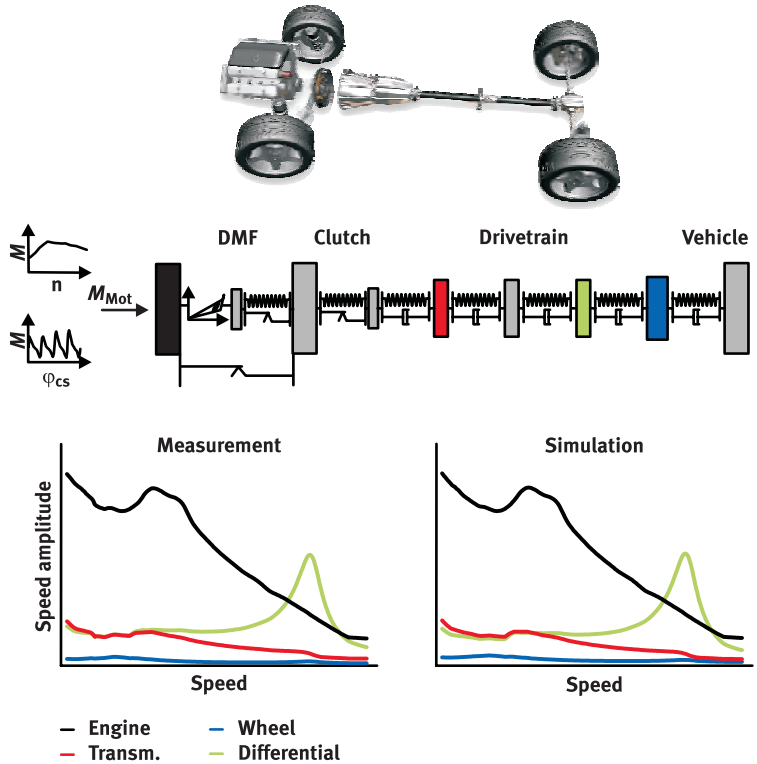
Figure 8 Full load in drive mode: analytical vibration model, measurement and simulation
