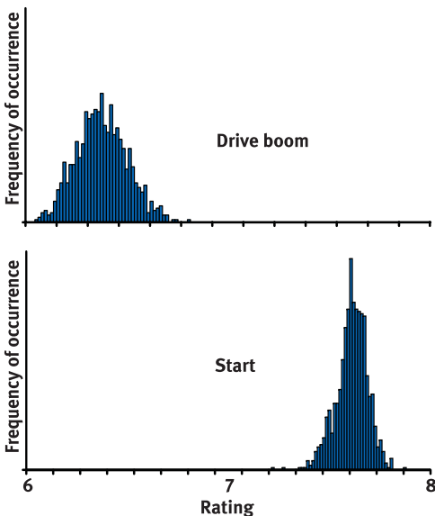
Figure 24 Distributions of the ratings for start and drive mode boom
