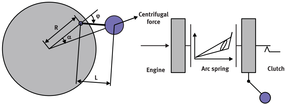
Figure 26 Functional arrangement of the centrifugal pendulum-type absorber
