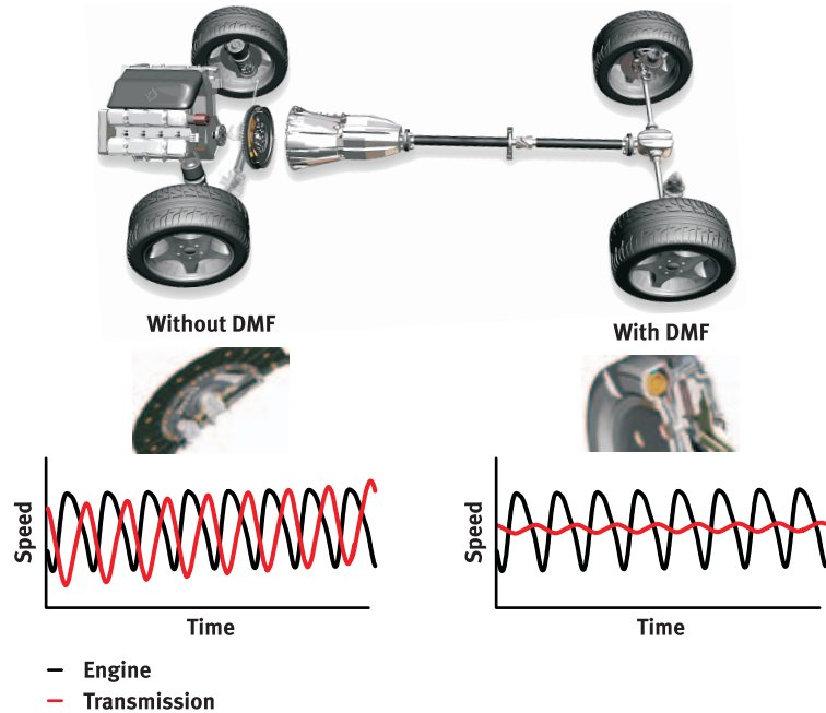
Figure 3 The effect of the DMF on comfort
