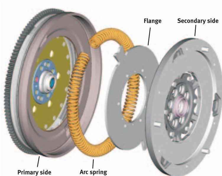
Figure 14 Components of a DMF
