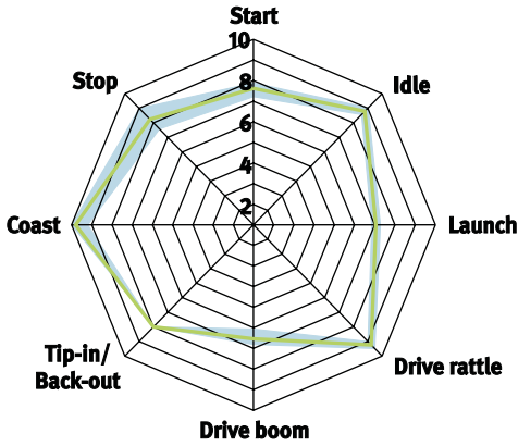
Figure 23 Results of the tolerance study
