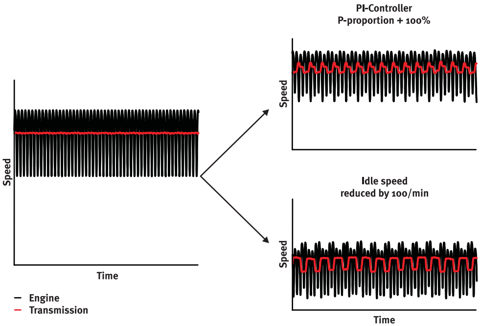
Figure 12 Idle: interaction between the DMF and engine management system
