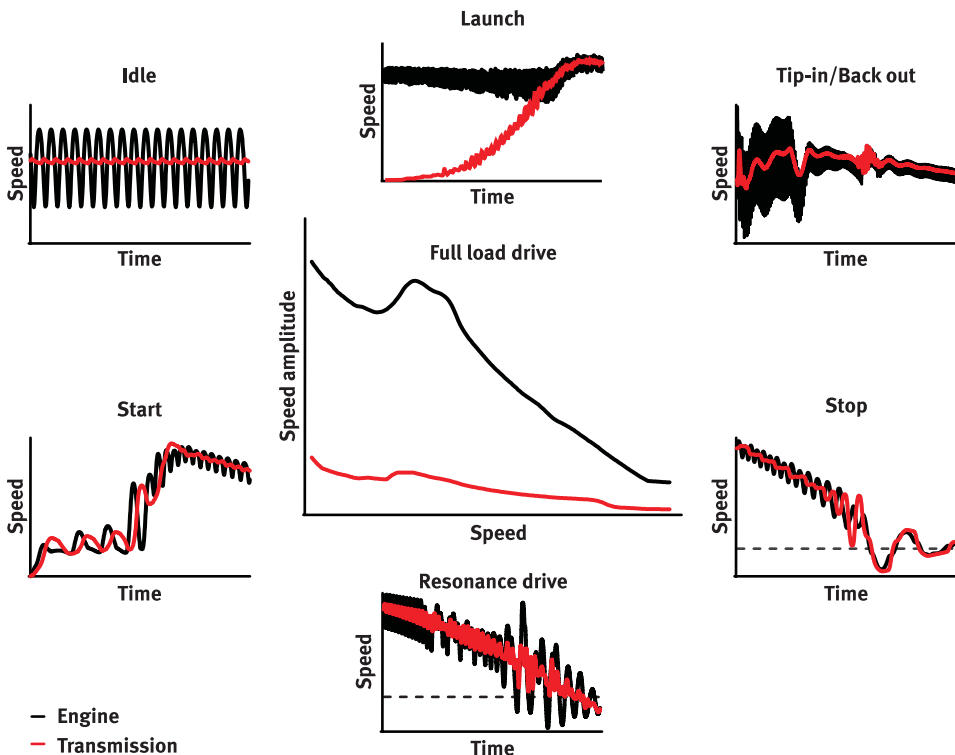
Figure 4 Important vehicle operating points
