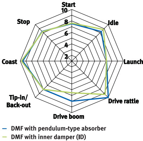
Figure 29 Comparison of optimization results of a conventional DMF with inner damper and a DMF with secondary-side centrifugal pendulum-type absorber
