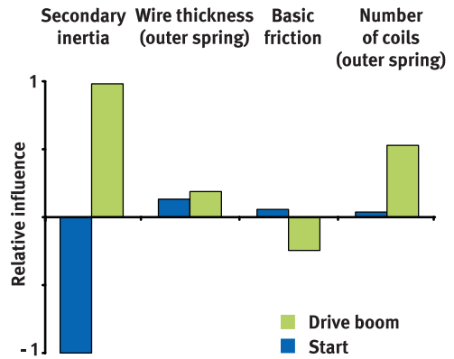
Figure 25 The most important influencing factors and their effects in relation to boom in drive mode and start behaviour
