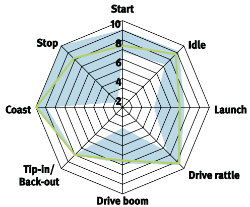
Figure 21 Optimization results for DMF with two-stage arc spring and inner damper
