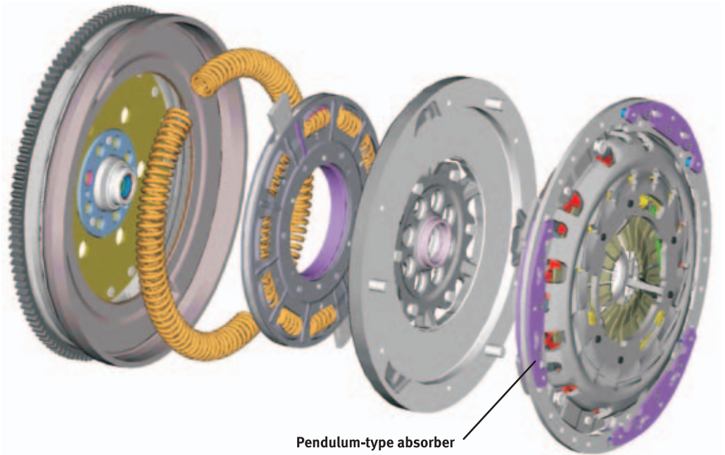
Figure 31 DMF with cover-side centrifugal pendulum-type absorber
