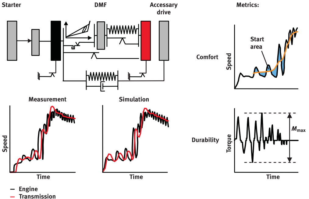
Figure 9 Engine start: analytical vibration model, measurement, simulation and metrics
