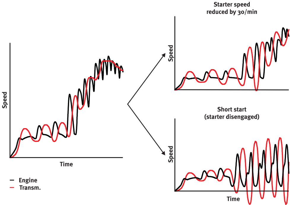
Figure 11 Engine start: Interaction of the DMF with the starter and engine management system
