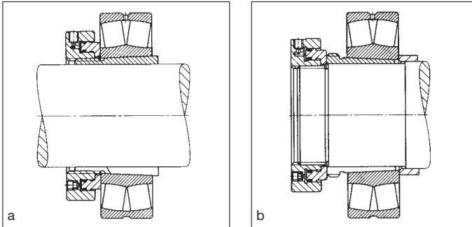
36: Mounting of a spherical roller bearing with an annular piston press.
