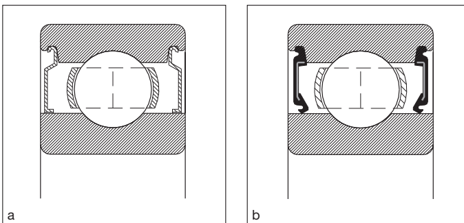
37: Never heat bearings with shields or seals in an oil bath. The maximum heating temperature is 80°C.
