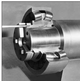
99: Dismounting a withdrawal sleeve mounted spherical roller bearing by the hydraulic method.
