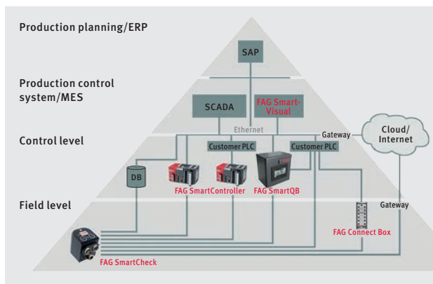
Integration of the FAG SmartCheck into the process landscape
